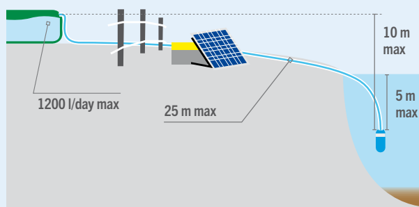
DIAGRAM: SOLAR-BASIC
